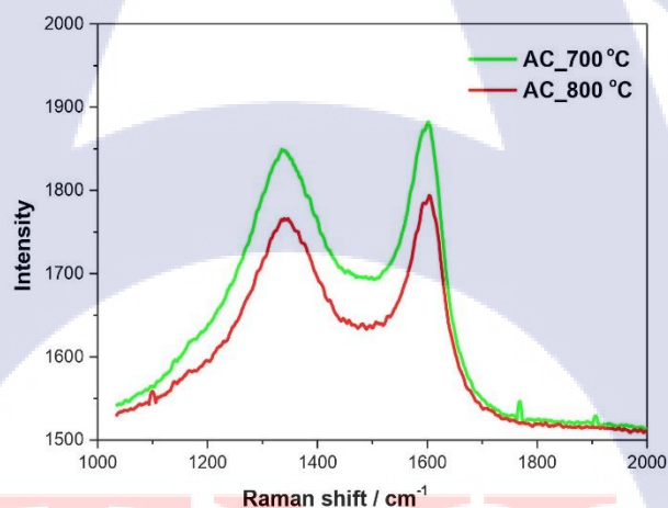
Figure 6. Raman spectra activated carbons prepared by calcining at 700 and 800 °C
