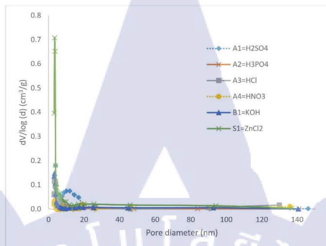
Figure 7. (b) The pore size distribution of activated carbon with different activating agents.
