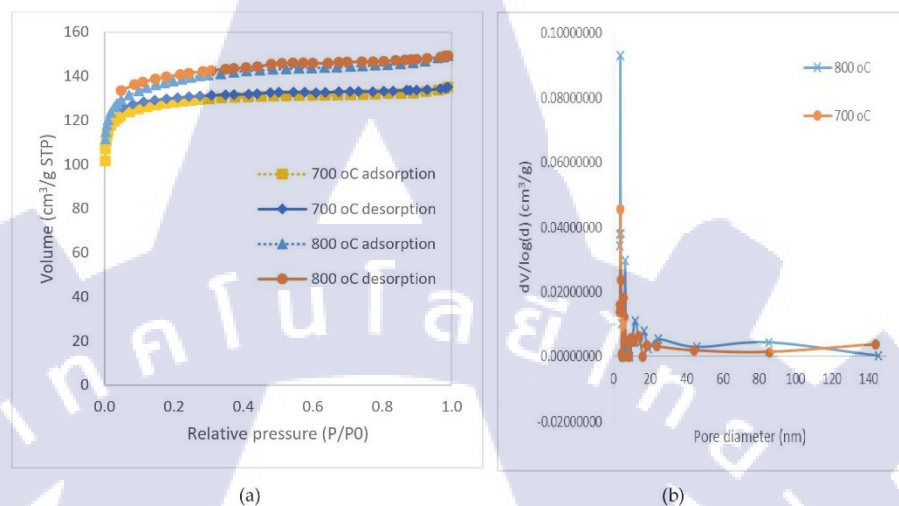
Figure 3. (a) Adsorption-desorption isotherm of activated carbon at 700 °C and 800 °C (b) The pore size distribution of activated carbon at 700 °C and 800 °C
