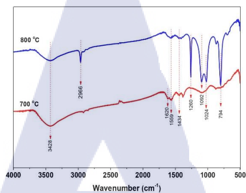
Figure 5. FT-IR spectra of activated carbon after activating at 700 °C and 800 °C
